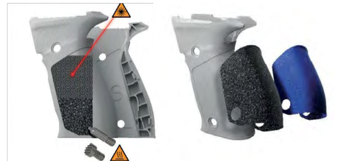
ATC SAO & DA/SA „BLANK“ GRIP 3S S/M/L DA/SA „BLANK“ GRIFF 3S S/M/L
